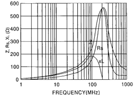
FI 76.2x28.5x12.7
