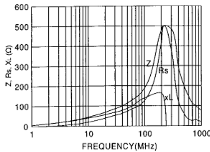
FI 63.5x28.5x12.7
